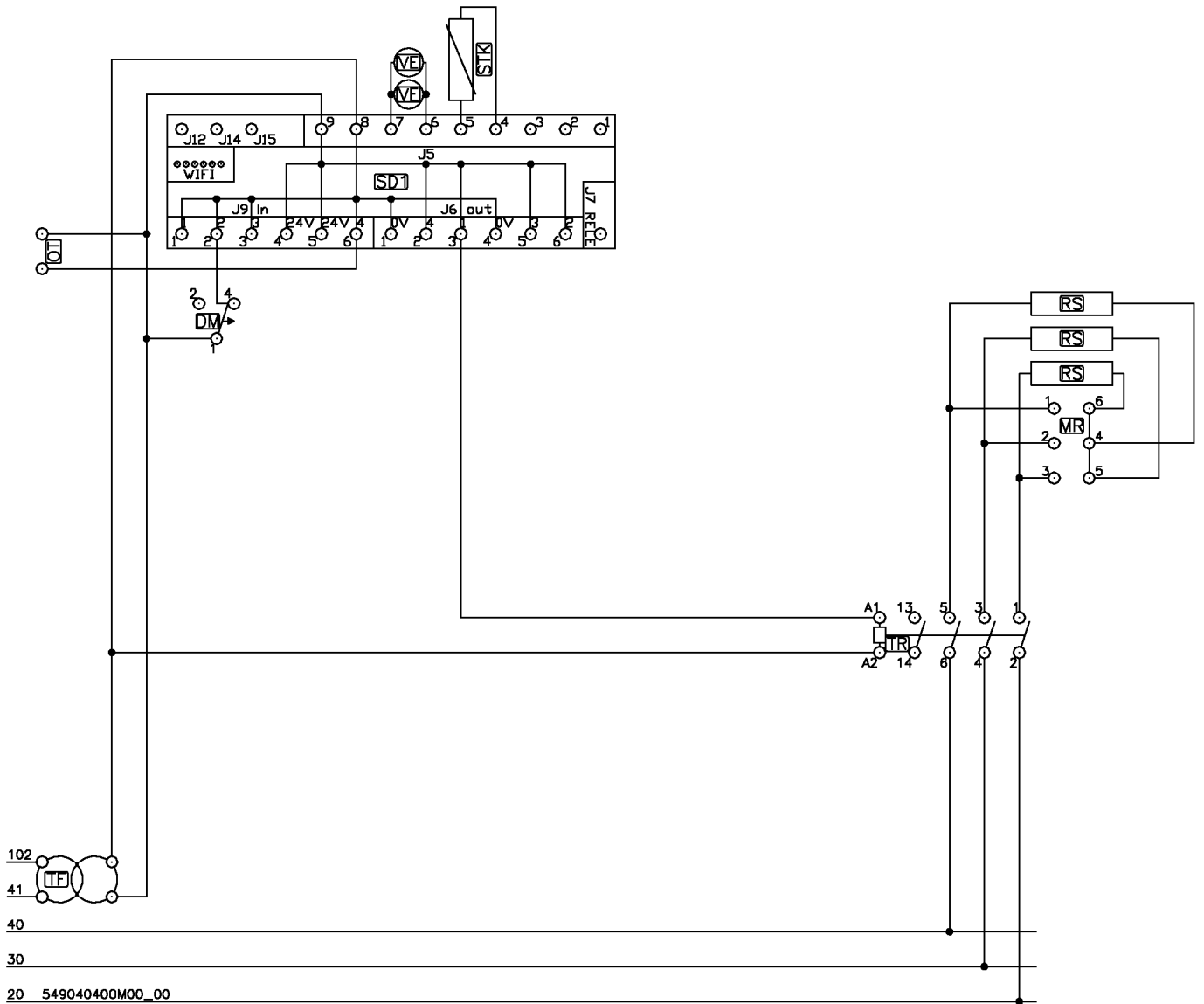
FIG. A WIRING DIAGRAM CWK-94ETT CWK-98ETT
