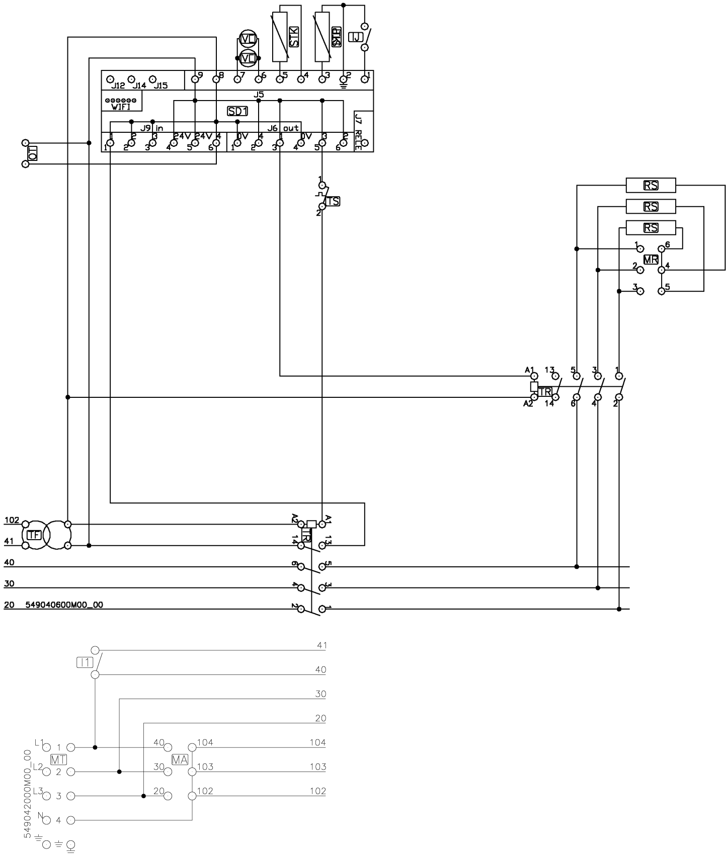
FIG. A WIRING DIAGRAM BRF-94ETT BRF-98ETT
